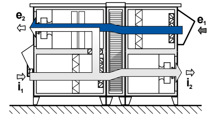
Combined mode (heat recovery mode with recirculation)
