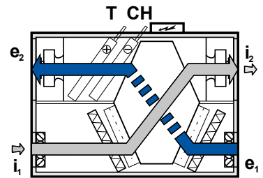
Bypass mode (without heat recovery)
