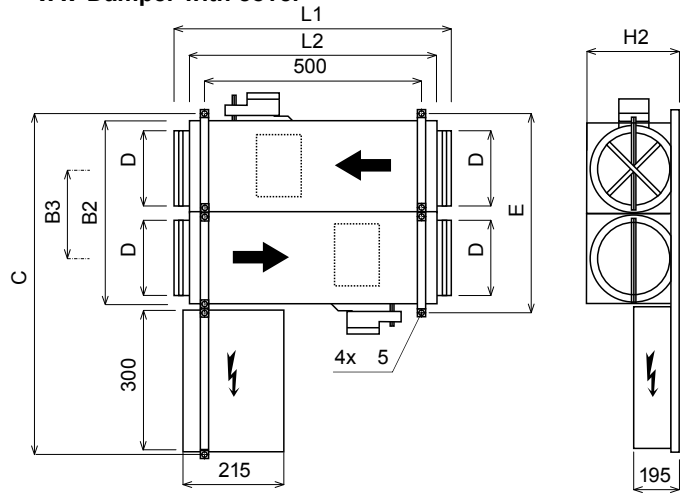
VAV Damper with cover
