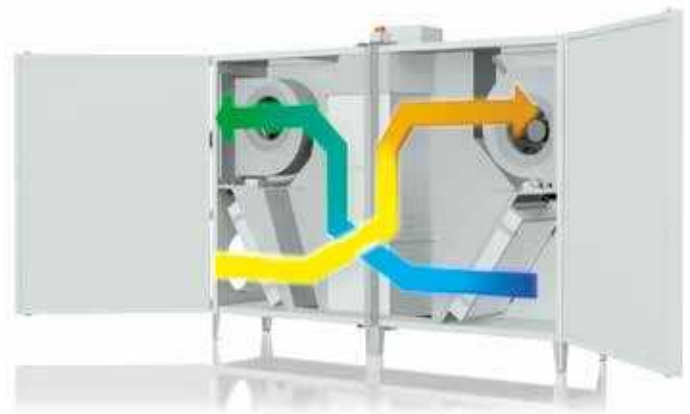
Interchangeable spigot design allows the spigot connections to be changed on-site (DV1600)
