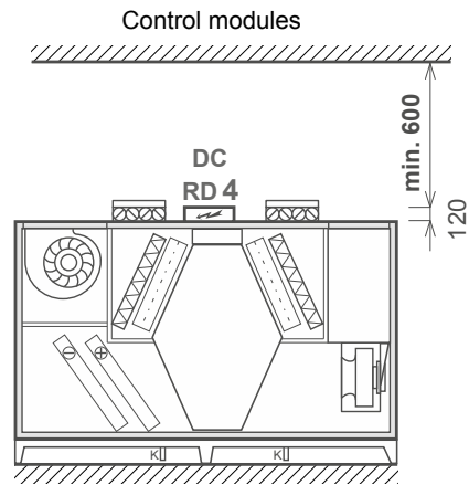
MANIPULATION SPACE FOR UNIT ACCESSORIES
