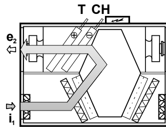
Recirculation mode with optional heating and cooling
