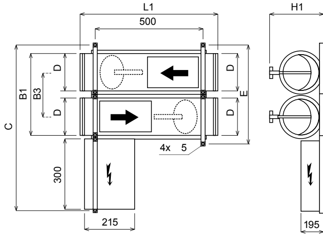
VAV Damper without cover
