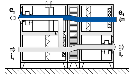
Combined mode (heat recovery mode with recirculation)
