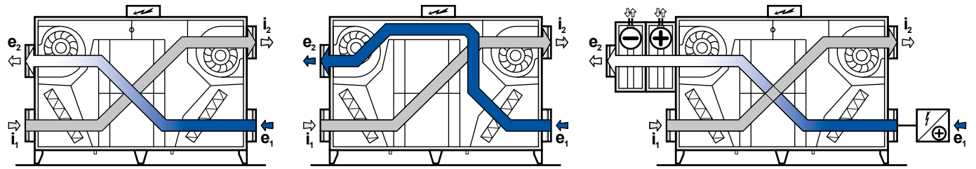
1. Equal pressure ventilation with heat recovery
