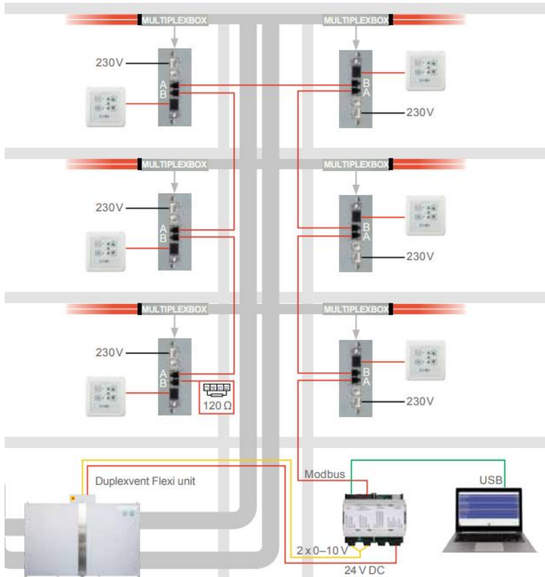
Figure 2: The Modbus Network commissioned from a single laptop using the Airflow Software!
